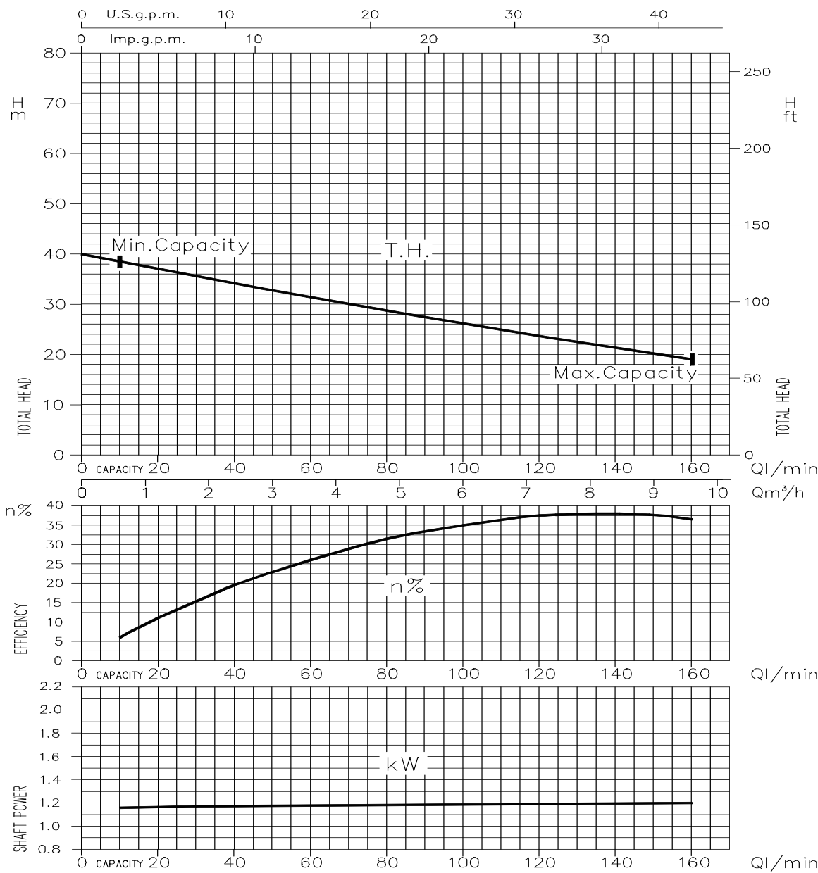
AGC 1.50 - Impeller diameter = 143 mm
