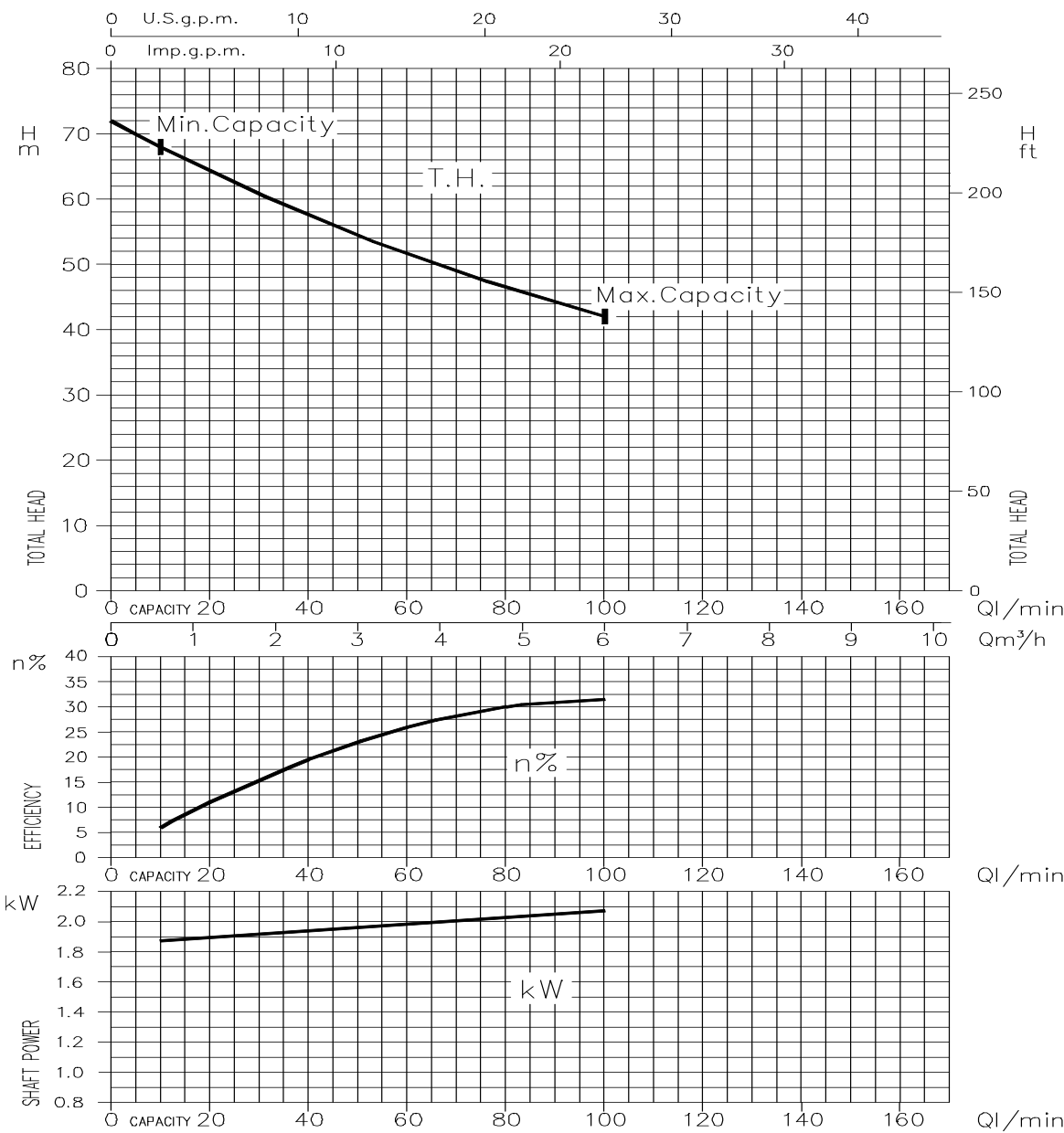
AGA 3.00 - Impeller diameter = 164 mm
